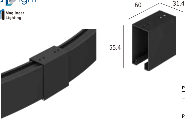
Connector
